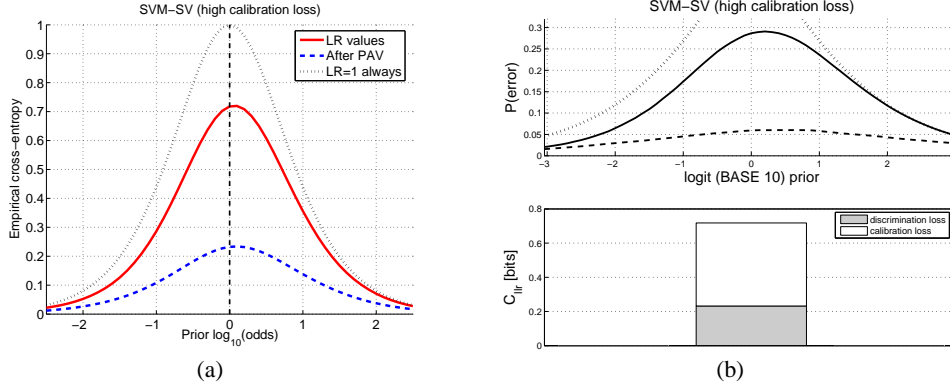
Figure 5: Comparison of the ECE plot (a) to APE plots and C_{urr} (b). ATVS SVM-SV system. NIST SRE 2006 protocol.
