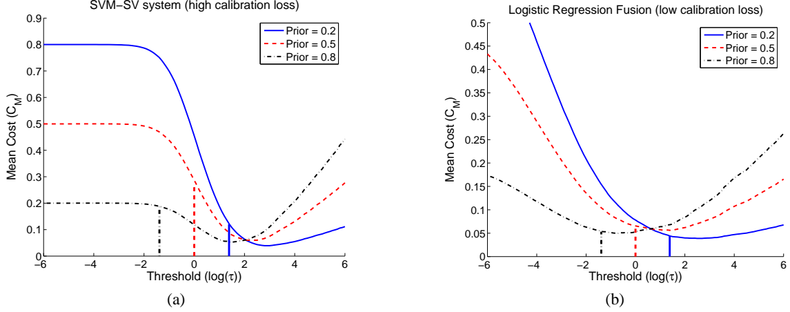
Figure 2: Value of C_M (Equation 3) for different decision thresholds. (a) SVM-SuperVector system (high calibration loss) and (b) Logistic regression fused system (low calibration loss). C_{f_r} = C_{f_a} = 1 . Bayes thresholds (Equation 5) are shown as vertical lines.
